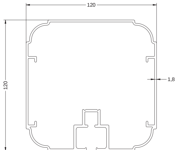
Ref.2674 GUÍA PÉRGOLA 120X120 MM
