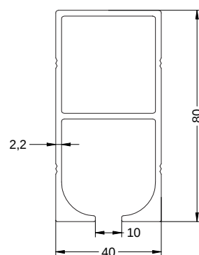
Ref.7805 GUÍA PÉRGOLA 80 MM
